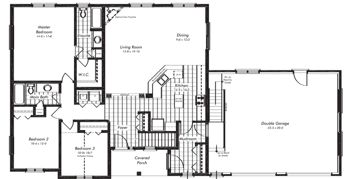
MAIN FLOOR PLAN Widetlot Option
