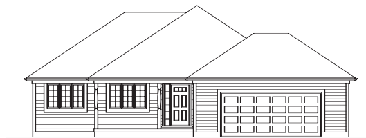
FRONT ELEVATION 'B'
