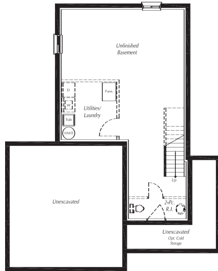
BASEMENT PLAN (All Elevations)
