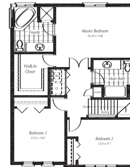
SECOND FLOOR PLAN - Elevation 'A' 3 Bedroom Option
