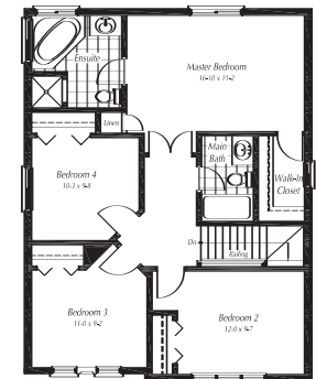
SECOND FLOOR PLAN - Elevation 'A' 4 Bedroom Option
