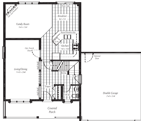
MAIN FLOOR PLAN - Elevation 'A'
